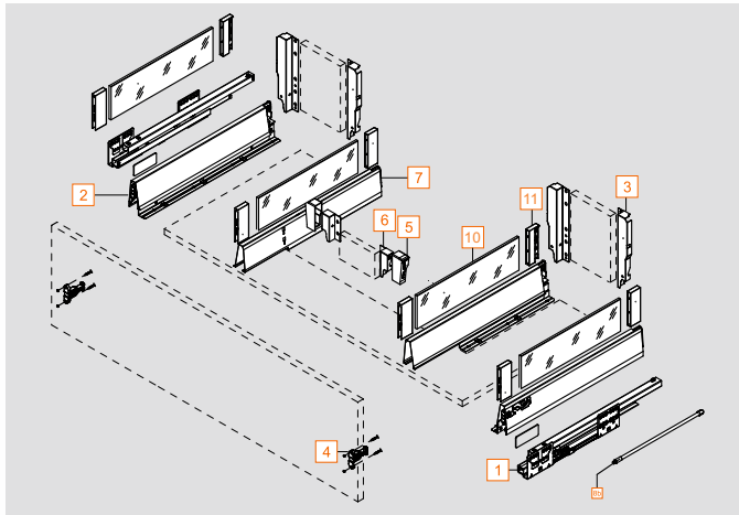
Under-Sink Drawer - Glass Gallery - 199mm
