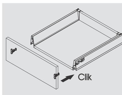
Fixing Front Panel
