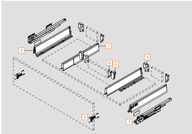
Under-Sink Drawer - 84mm Height
