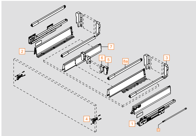
Under-Sink Drawer - Single Gallery - 135mm
