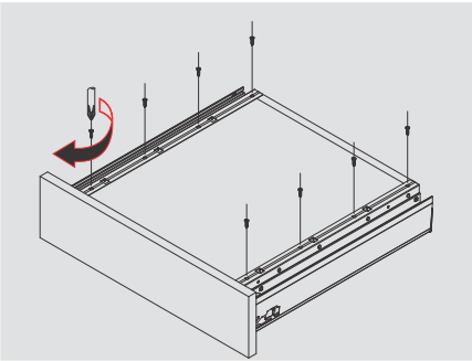
Fix Screws
