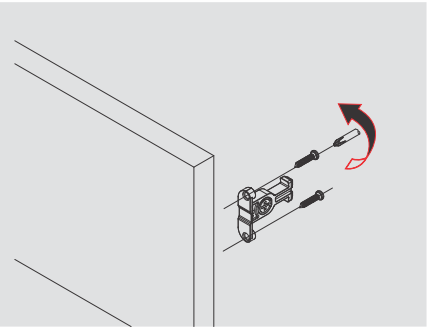
Front Assembly
