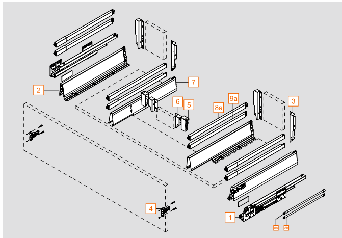
Under-Sink Drawer - Double Gallery - 199mm
