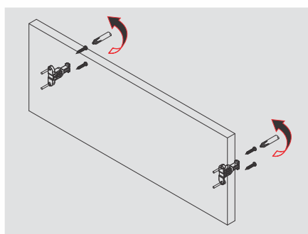
Front Assembly
