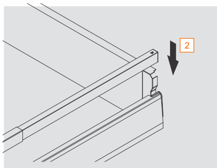
Back Assembly
