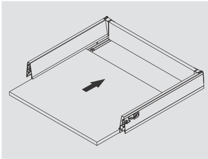
Bottom Assembly
