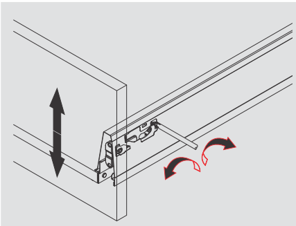
Up - Down Adjustment
