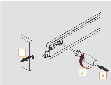
Turn screw driver to release the drawer
